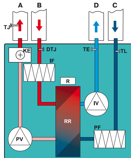
LV-RACU 700, 1200 VER-V4
