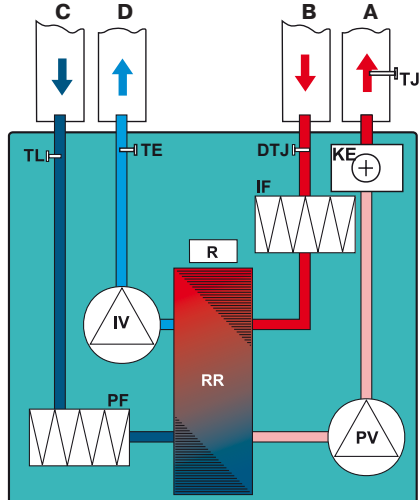
LV-RACU 700, 1200 VEL-V4
